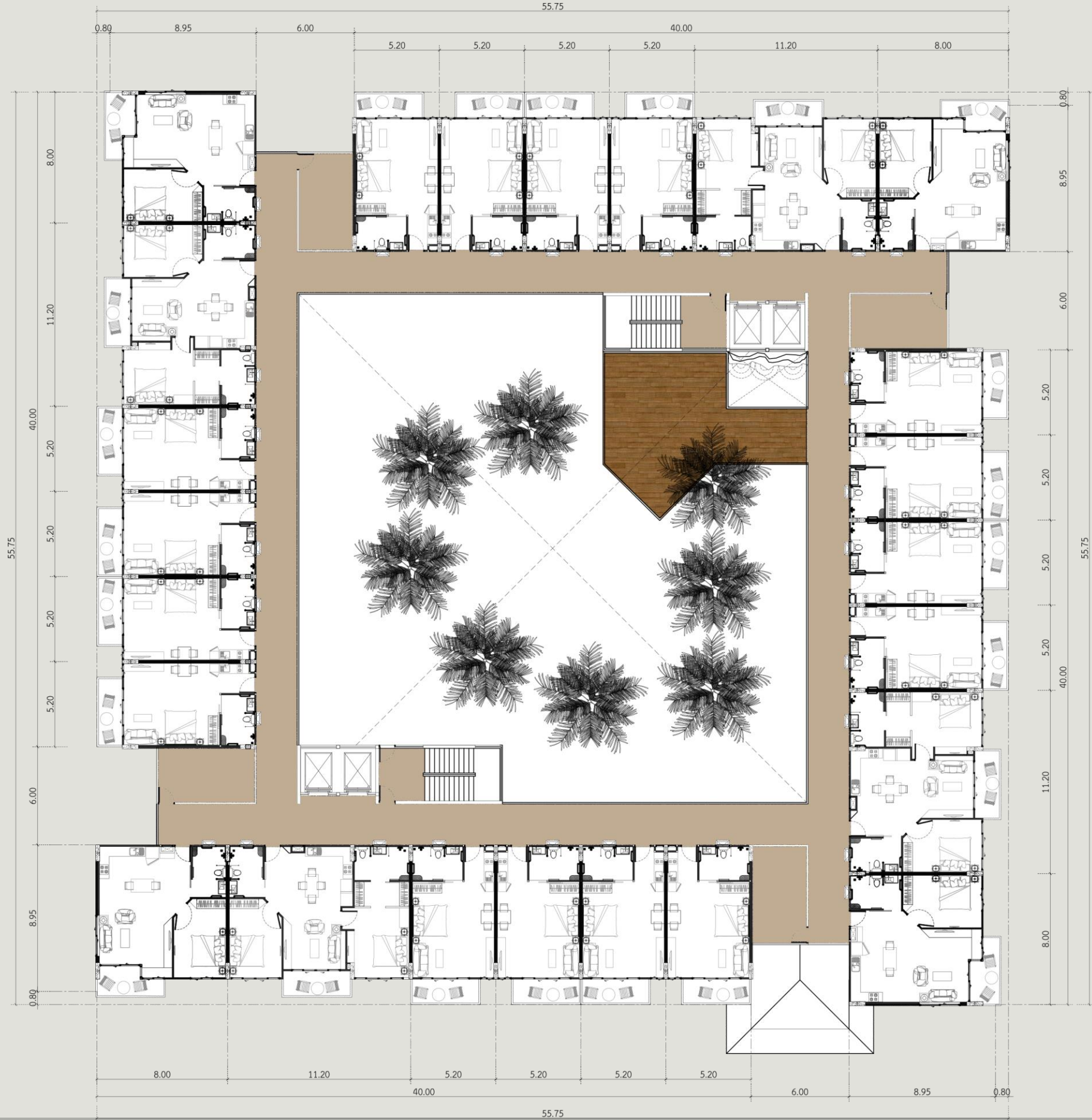
APARTMENT 1 ST FLOOR PLAN
