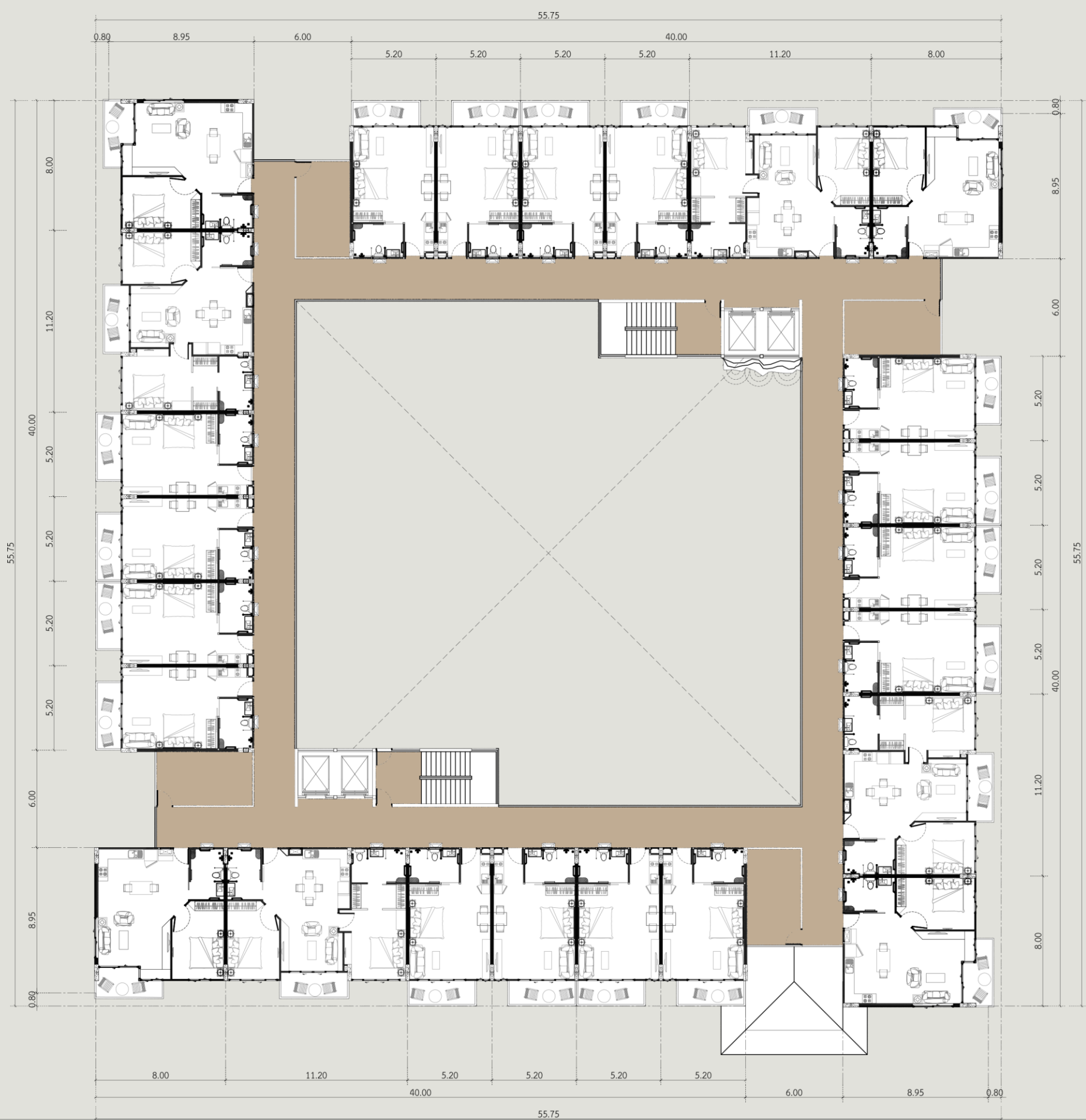
APARTMENT 2 ND FLOOR PLAN PLAN
